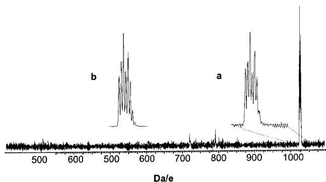
Figure 2. Negative-ion mode ES mass spectrum of \text{PPN}[\text{CpW}(\text{CO})_2(\text{C}_{60})] : (a) observed; (b) calculated
