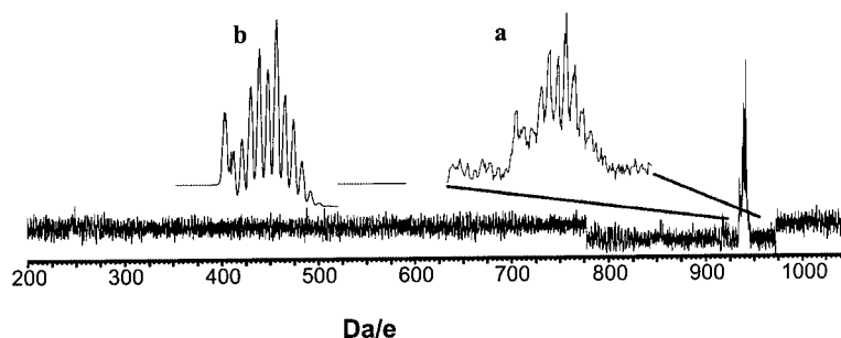
Figure 1. Negative-ion mode ES mass spectrum of PPN[CpMo(CO) 2 (C 60 )]: (a) observed; (b) calculated
