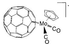
Figure 3. Proposed Structure of the [\text{CpMo}(\text{CO})_2(\text{C}_{60})]^- anion
